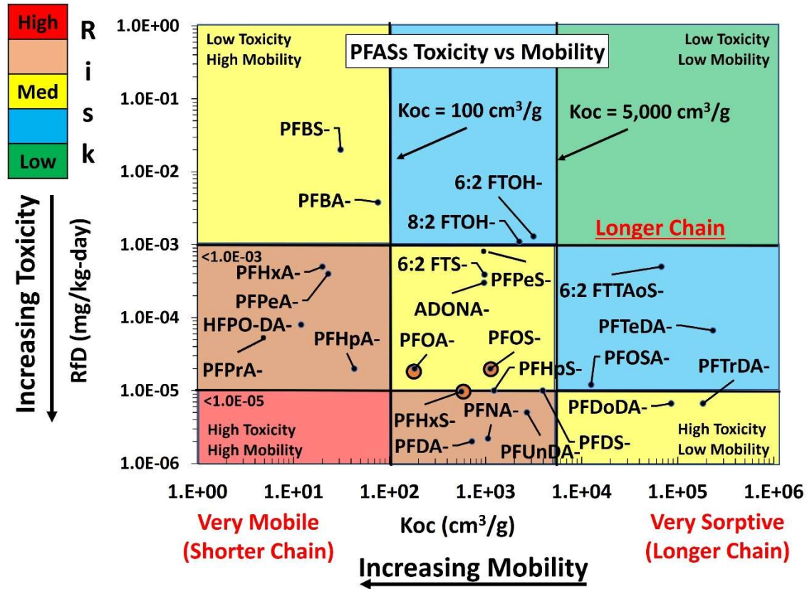
Figure 8. Comparison of PFASs mobility versus toxicity.
