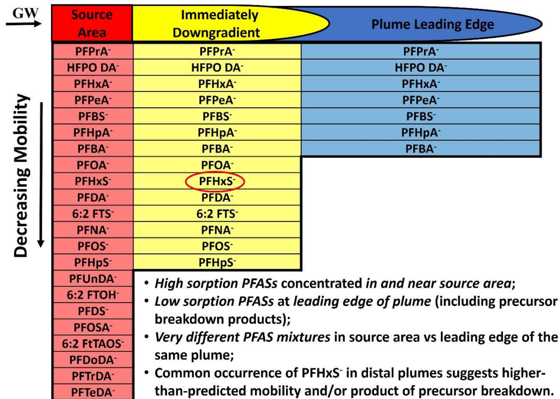
Figure 7. Hypothetical PFASs groundwater plume separation based on sorption coefficients for individual compounds.
